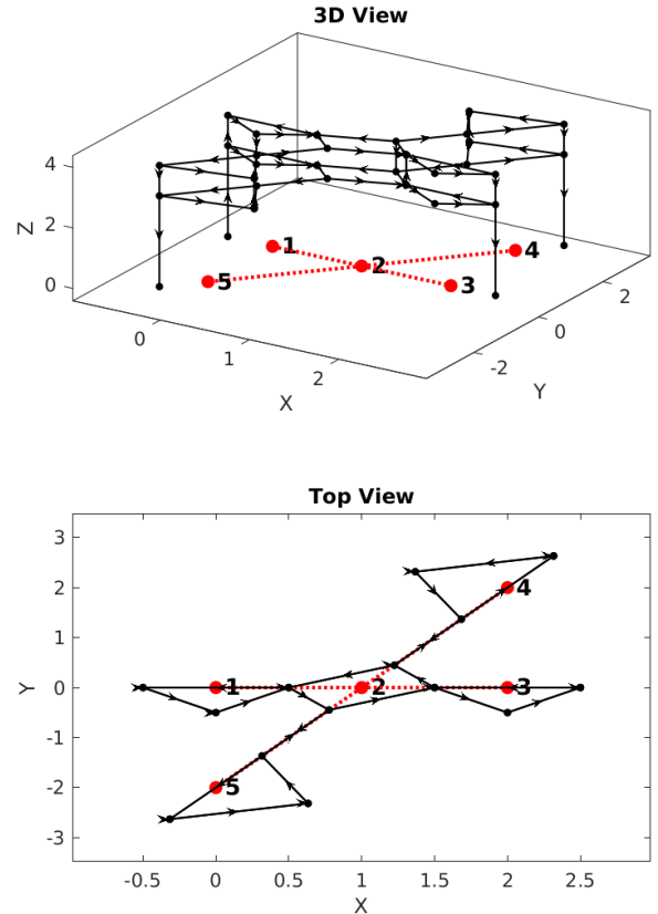
Fig. 2. Roundabout Formation Around Ground-Vertex v_0
