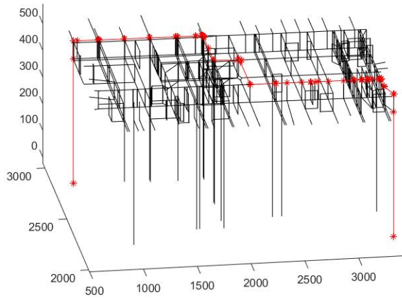
Fig. 9. Airway Path Corresponding to Ground Path.
