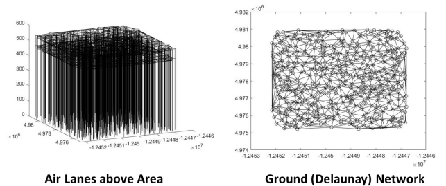
Fig. 12. Lanes Constructed from Delaunay Triangulation (left: airways; right: ground network).
