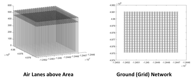
Fig. 11. Lanes Constructed from Rectangular Grid (left: airways; right: ground network).
