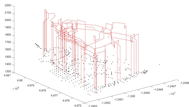
Fig. 1. Selected UAS Paths in a Lane Network over Salt Lake City, UT.
