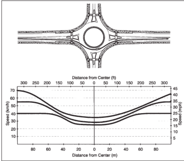
Recommended maximum entry design speeds for roundabouts at various intersection site categories are provided in Exhibit 6-4.
