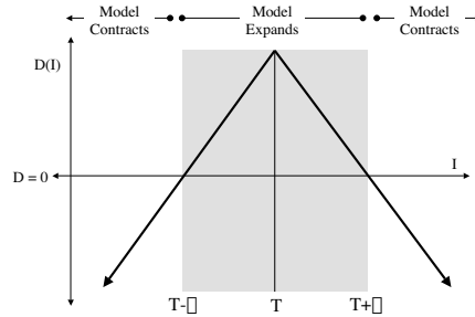
Figure 7: A speed function based on image intensity causes the model to expand over regions with greyscale values within a certain range and contract otherwise.
